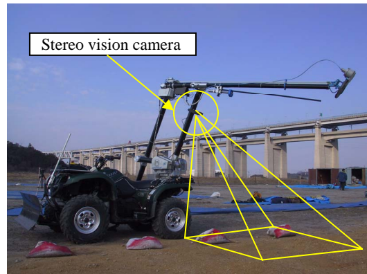
Fig. 7. The arm can be lifted up and controlled to different postures for effective topographical map acquisition.
