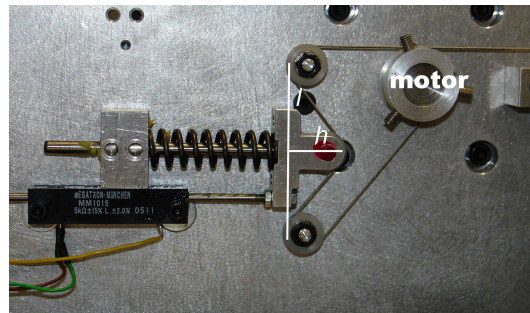
Fig. 2 Setup for a biarticulate joint with a nonlinear spring. Height h of the triangle relative to l/2 determines the stiffness constant.
