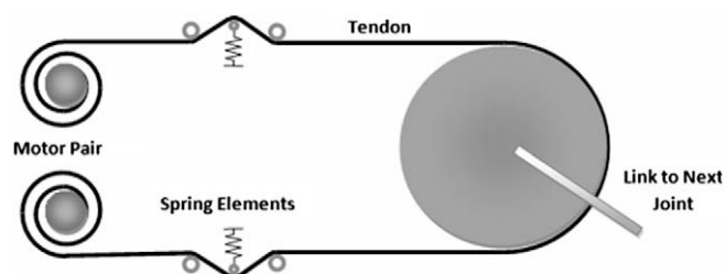
Fig. 4. Biarticulate control of a joint using non-linear spring elements. The height of the spring determines the stiffness constant.
