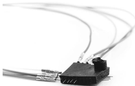
Fig. 16. 11 × 11 mm prototype of the “dermal” sensor.
