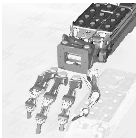
Fig. 8. Rendering of DLR's hand–arm system.
