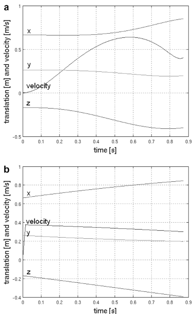
Fig. 20. Catching movement in x, y and z direction and tangential velocity of the hand for (left) the human-like and (right) purely technical catching strategies.
