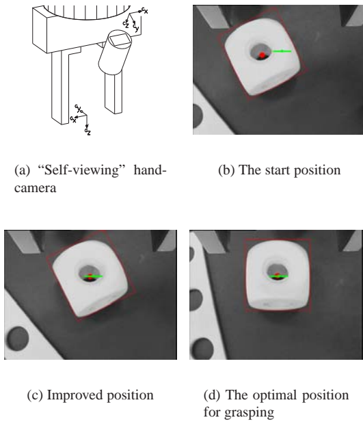
Figure 7. Fine-Positioning using a "self-viewing" hand-camera.
