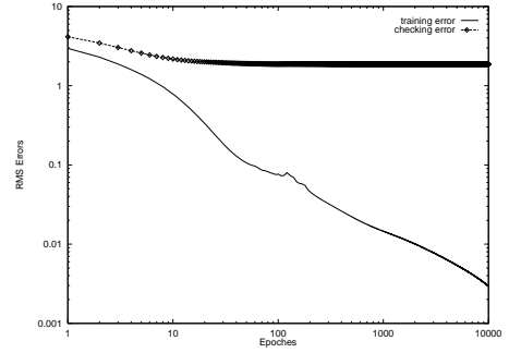
Figure 6. RMS errors of modelling the Box-Jenkins data with four eigenvectors. 148 data are used for training and 148 data for checking.
