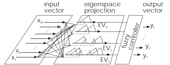
Figure 2. The structure of a fuzzy controller based on eigenspace projection.
