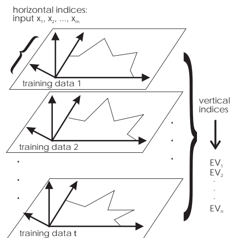
Figure 1. Vertical information about the distribution of the data in the input space can be extracted by statistics on a sequence of the training data set.
